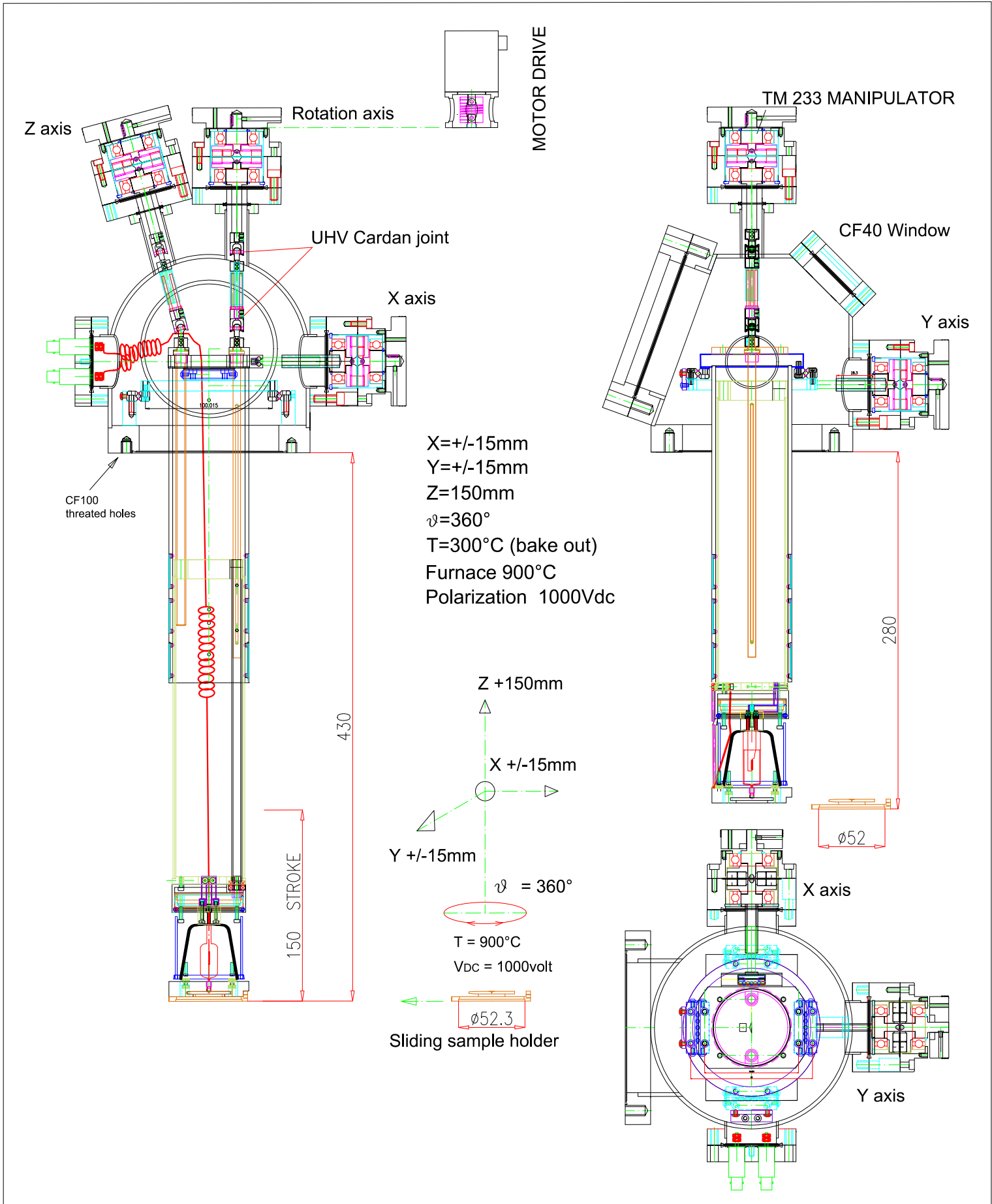
fig. 4 X-Y-Z Manipulator Mod XY15Z150TφV
